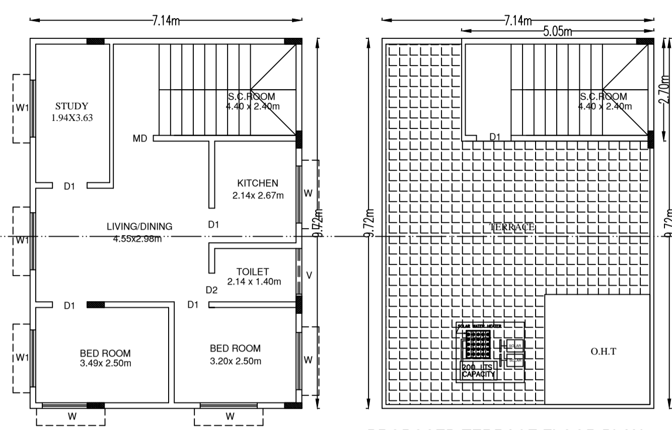
PROPOSED TERRACE FLOOR PLAN
